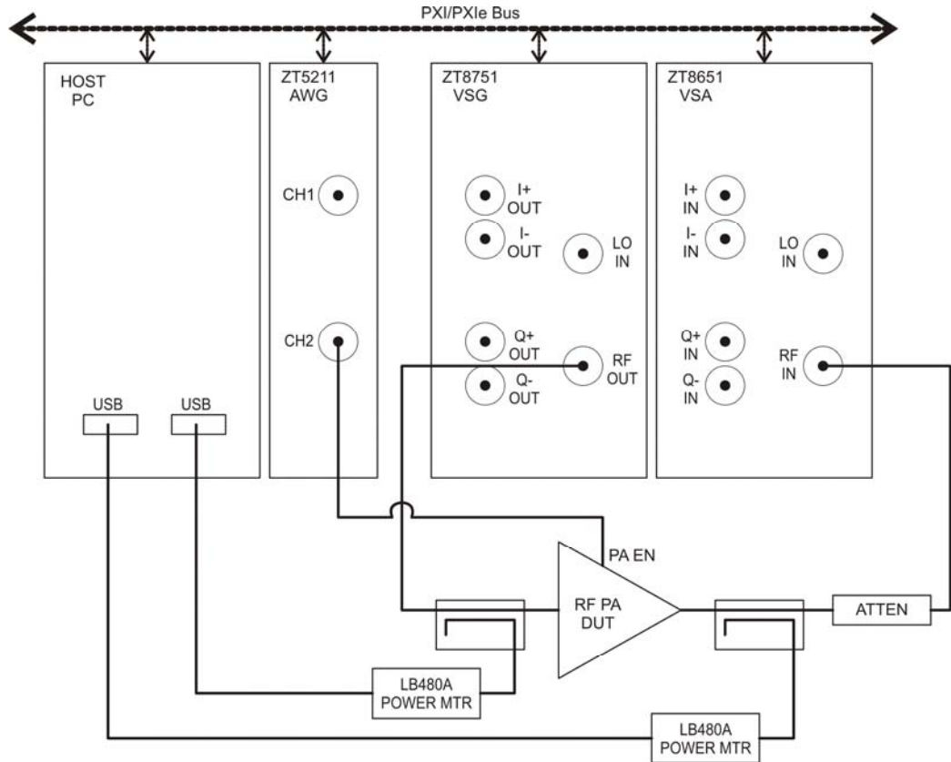
Figure 1) Test equipment block diagram for PA testing
