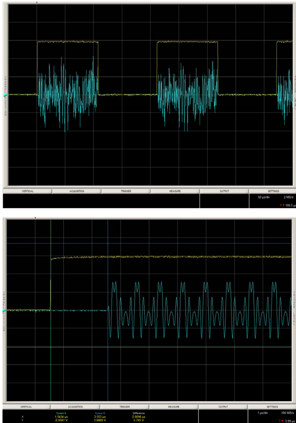
Figure 3) Time Domain Plots of PA Enable (yellow) and RF Pulse (blue)
