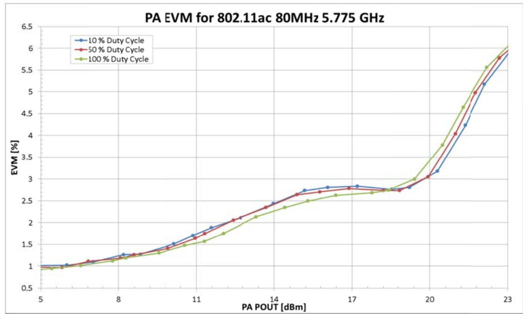
Figure 4) PA Dynamic EVM versus Duty Cycle
