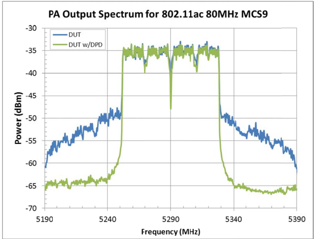
Figure 5) PA Adjacent Channel Leakage Reduction with DPD
