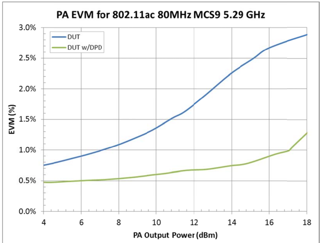
Figure 6) PA EVM Improvement with DPD
